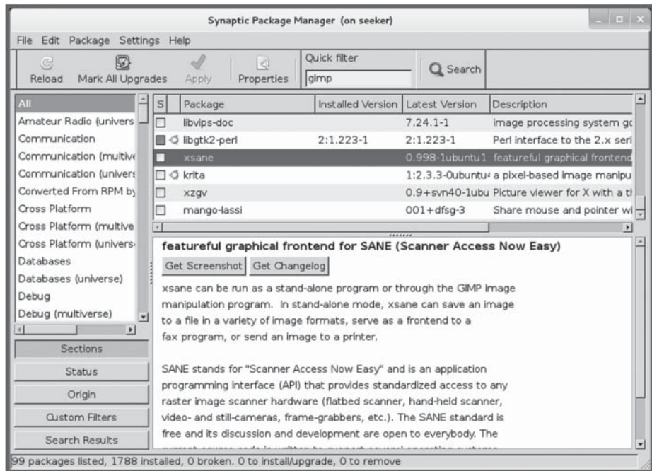
FIGURE 9.2 Synaptic enables you to search for, select, install, and uninstall software on Debian-based systems.
