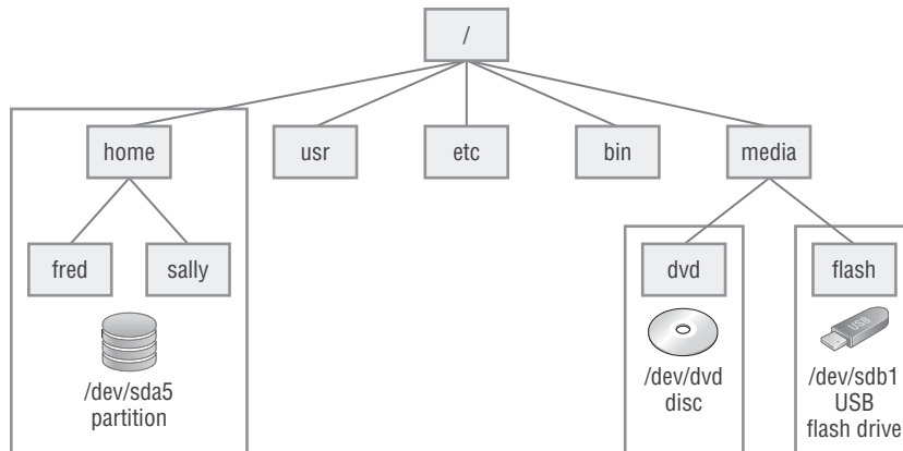
FIGURE 7.2 In Linux, all files are referenced relative to a single root (/) directory.
